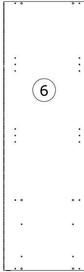
FB01753 1333x402x16mm
