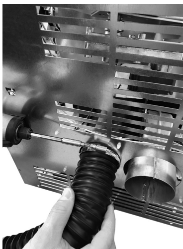
Fig. 12 - Raccordement air comburant
