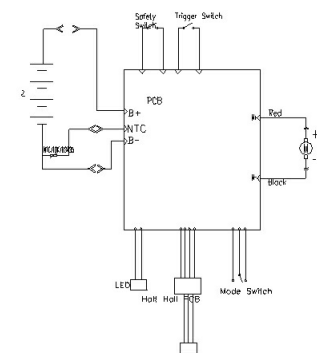
Electric Circuit
