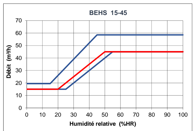
Figure 24 – HB04 – BEHS 15-45 (20-50%HR)
