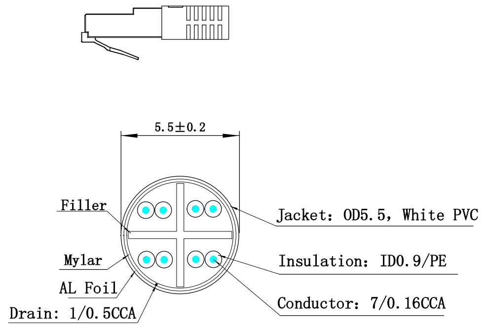
cable structure
