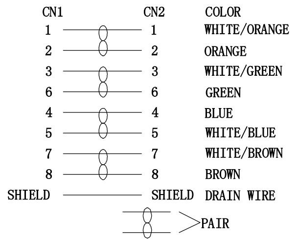
wiring diagram
