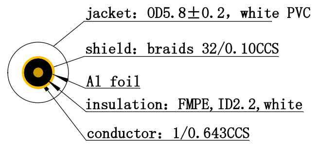
cable structure
