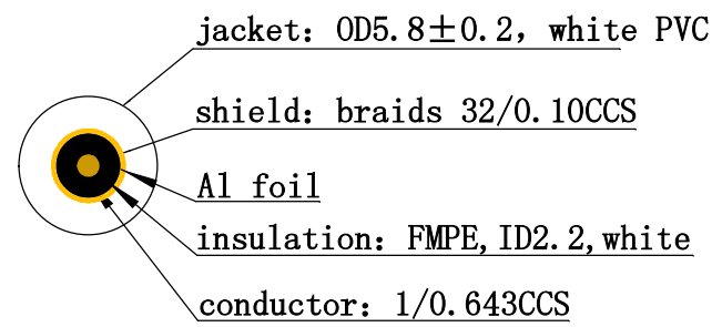
cable structure
