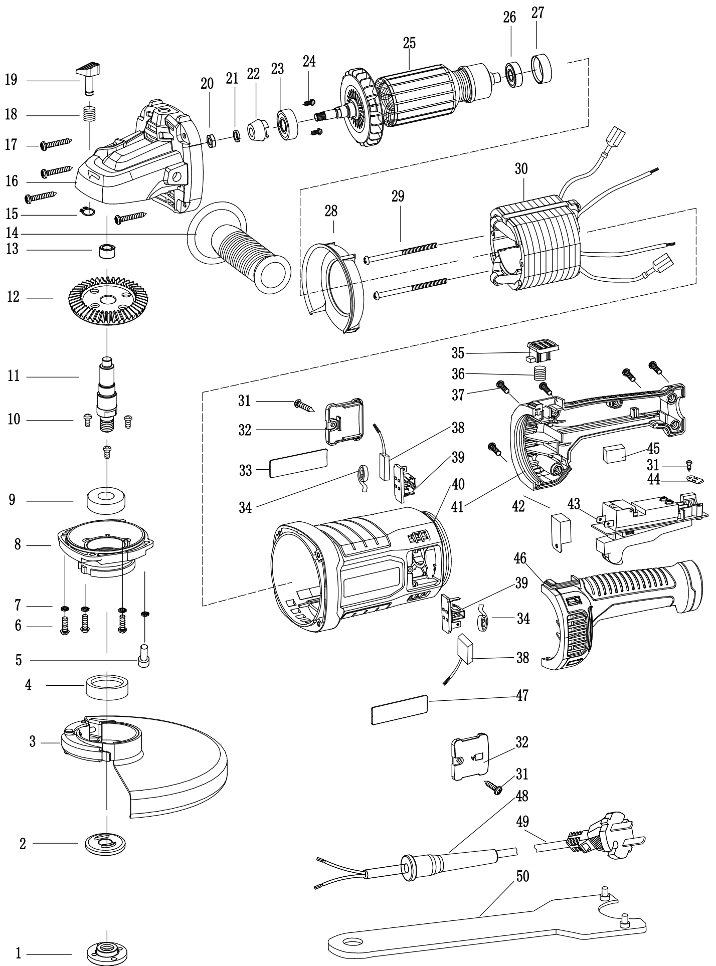
2100AG2-230.5 Exploded view
