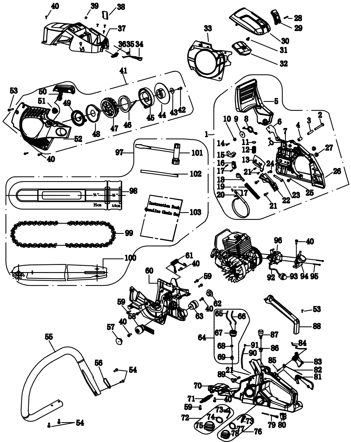
PCS2-35.31 base unit
