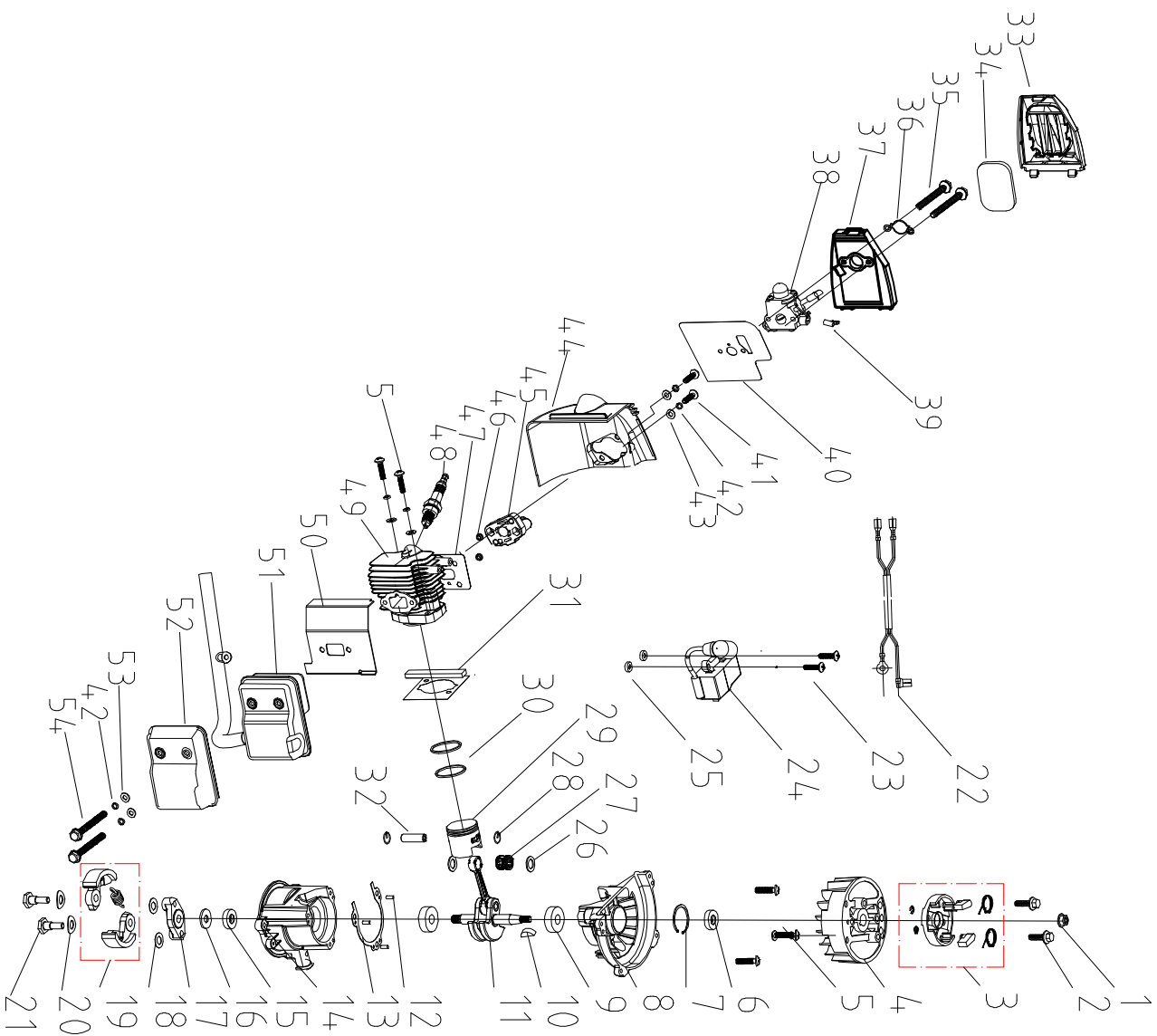
PHT1-60.21 Engine unit
