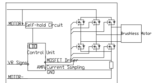
Electric Circuit
