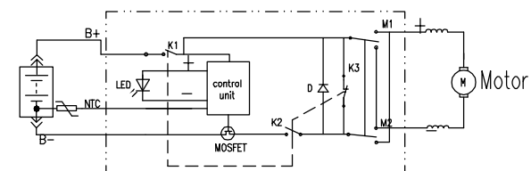
Electric circuit
