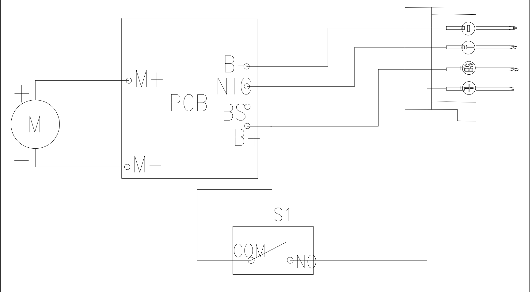
Electric circuit
