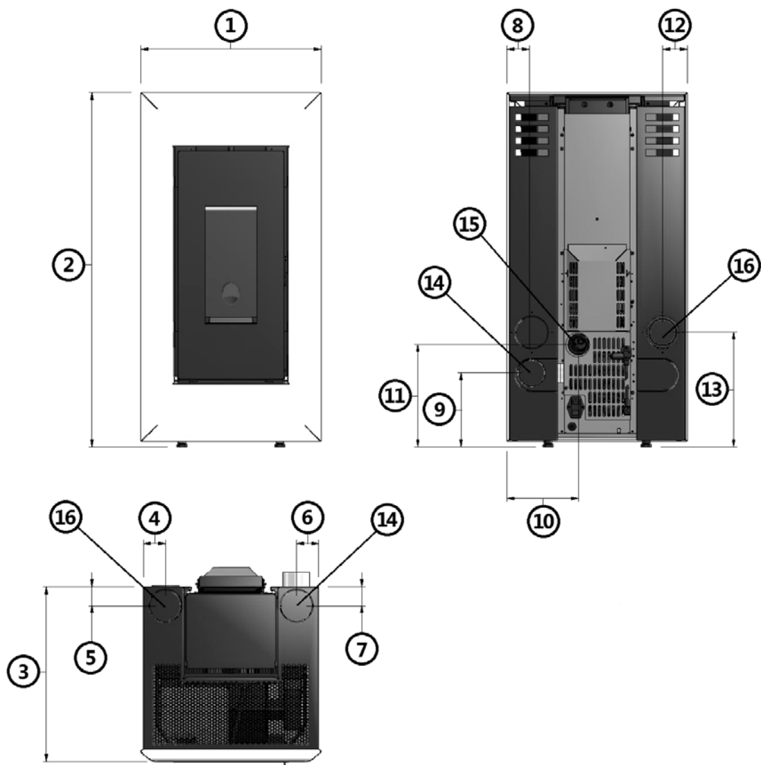
Fig. 29 - Dimensions générales: Vega At / Trend At
