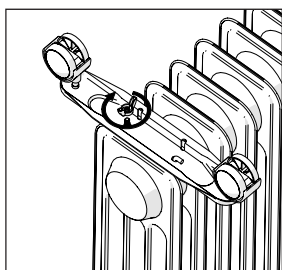
5 - Tighten using the wing nut
